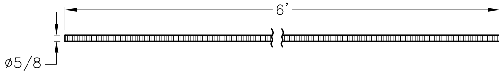
6' THREADED ROD
